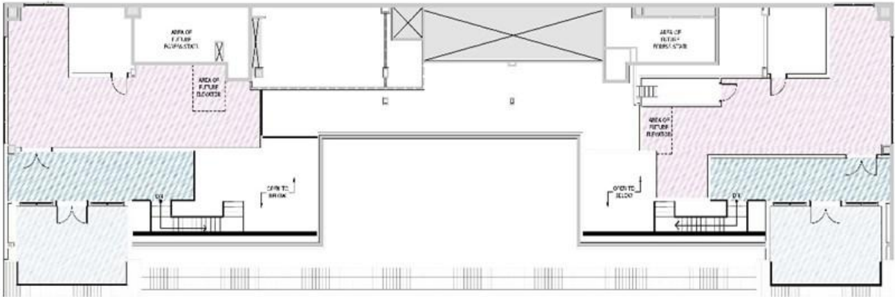
LEVEL 15M FLOOR PLAN - NEW Scale: 1/8" = 1'-0"
