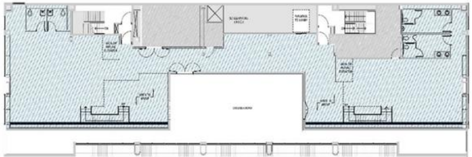
LEVEL 15 FLOOR PLAN - NEW Scale: 1/8" = 1'-0"
